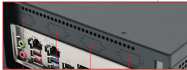
4 cutouts reserved for 4 x COM Ports
