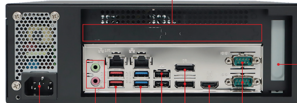
ATX Power Input Line-in and Line-out 4 x USB 3.2 and 2 x RJ45 LAN Ports 2 x USB 2.0 2 x DP HDMI 2 x COM Ports
